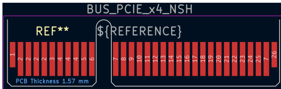
Figure 2: footprint-pcie
