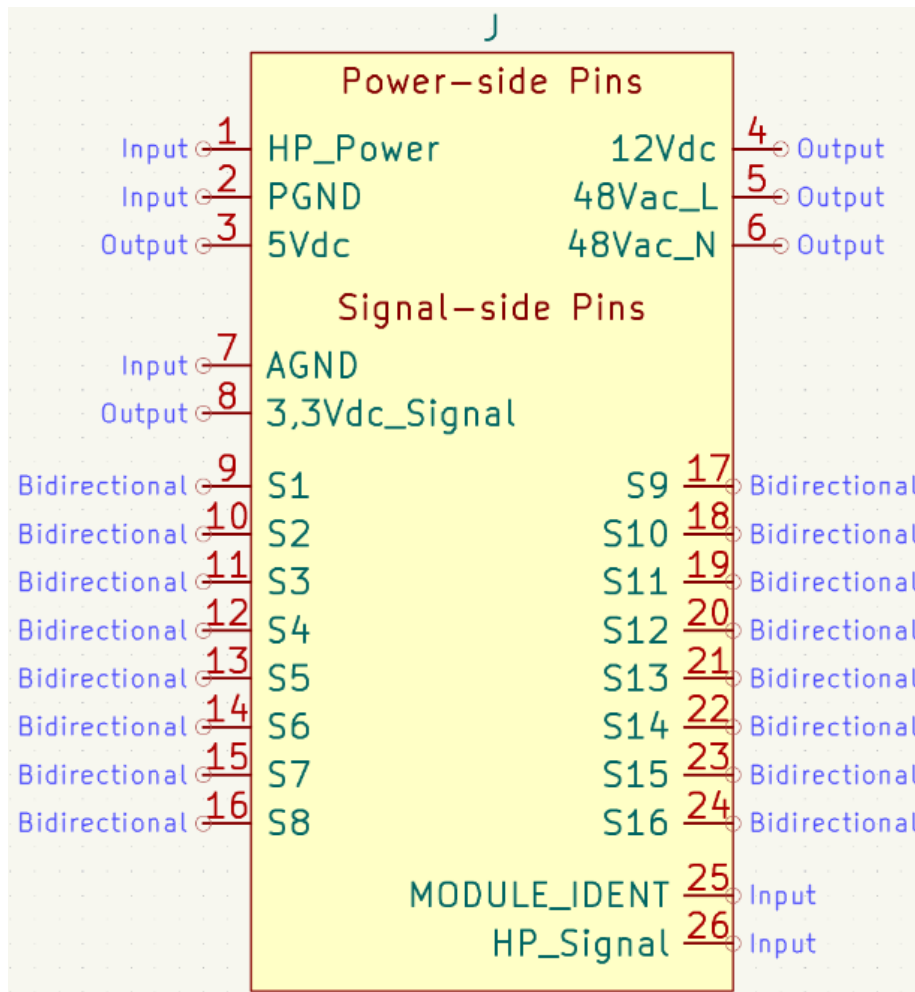
Figure 1: simbolo-pcie
