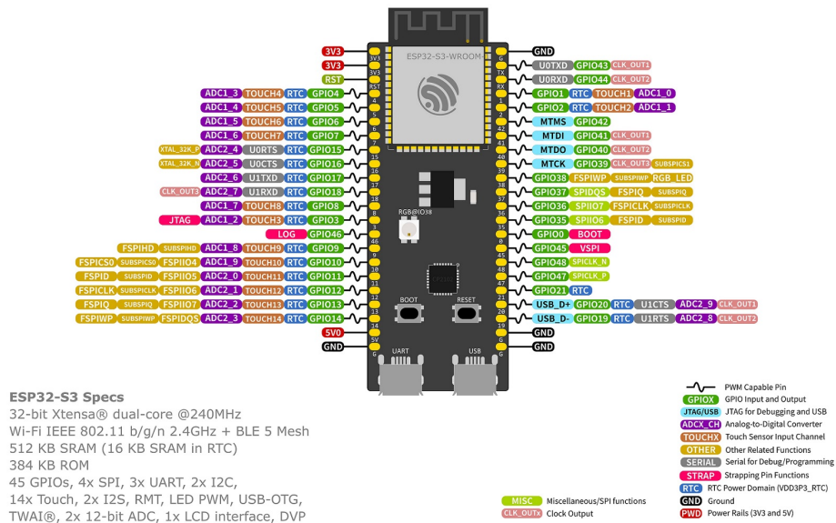
Figure 3: pinout-esp32
